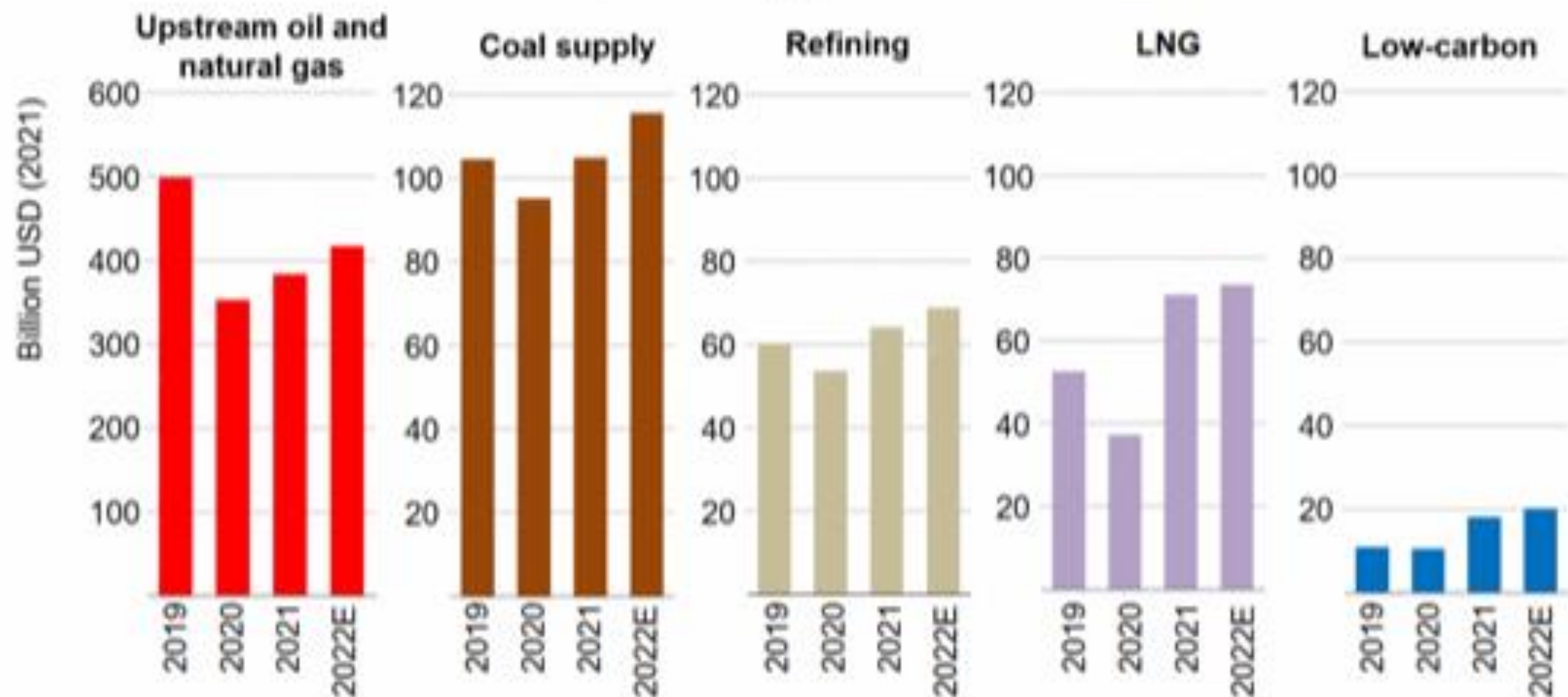
Change in fuel supply investment 2019-22
